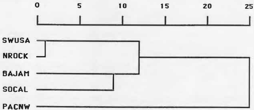
FIG. 6.—Dendrograms produced by cluster analysis (UPGMA, Euclidean distance) of mean values of 15 dependent variables, sexes combined, in sample groups one to four and milleri from Baja, California, México. Horizontal bar indicates rescaled morphometric differences between groups.
