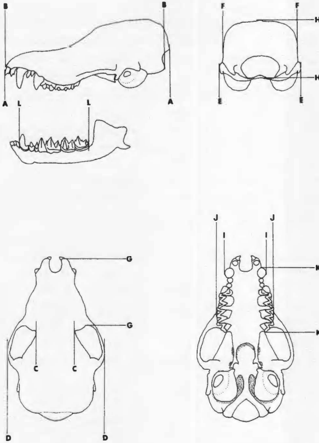
FIG. 1.—Lateral (cranium and dentary), posterior, dorsal and ventral aspect of skull of adult female M. evotis (TTU 38734) from Socorro County, New Mexico. Letters correspond to measurements in text.
