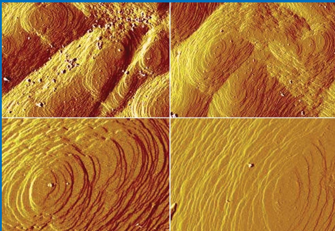
Effect of zinc doping on pentaerythritol tetranitrate single crystals (G. Zhang, S. K. Bhattacharia, and B. L. Weeks, p. 732)
