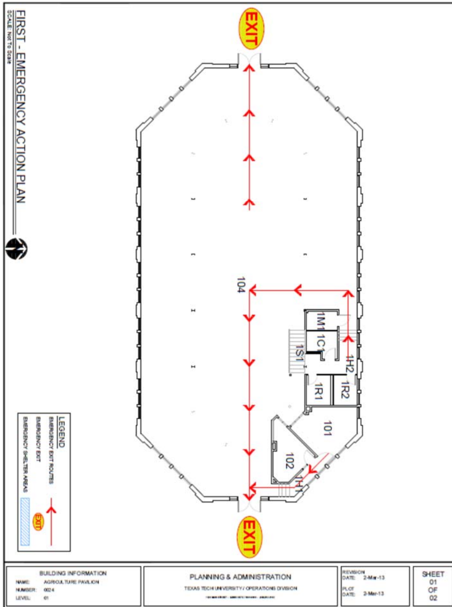
Figure 5 Agricultural Pavilion First Floor
