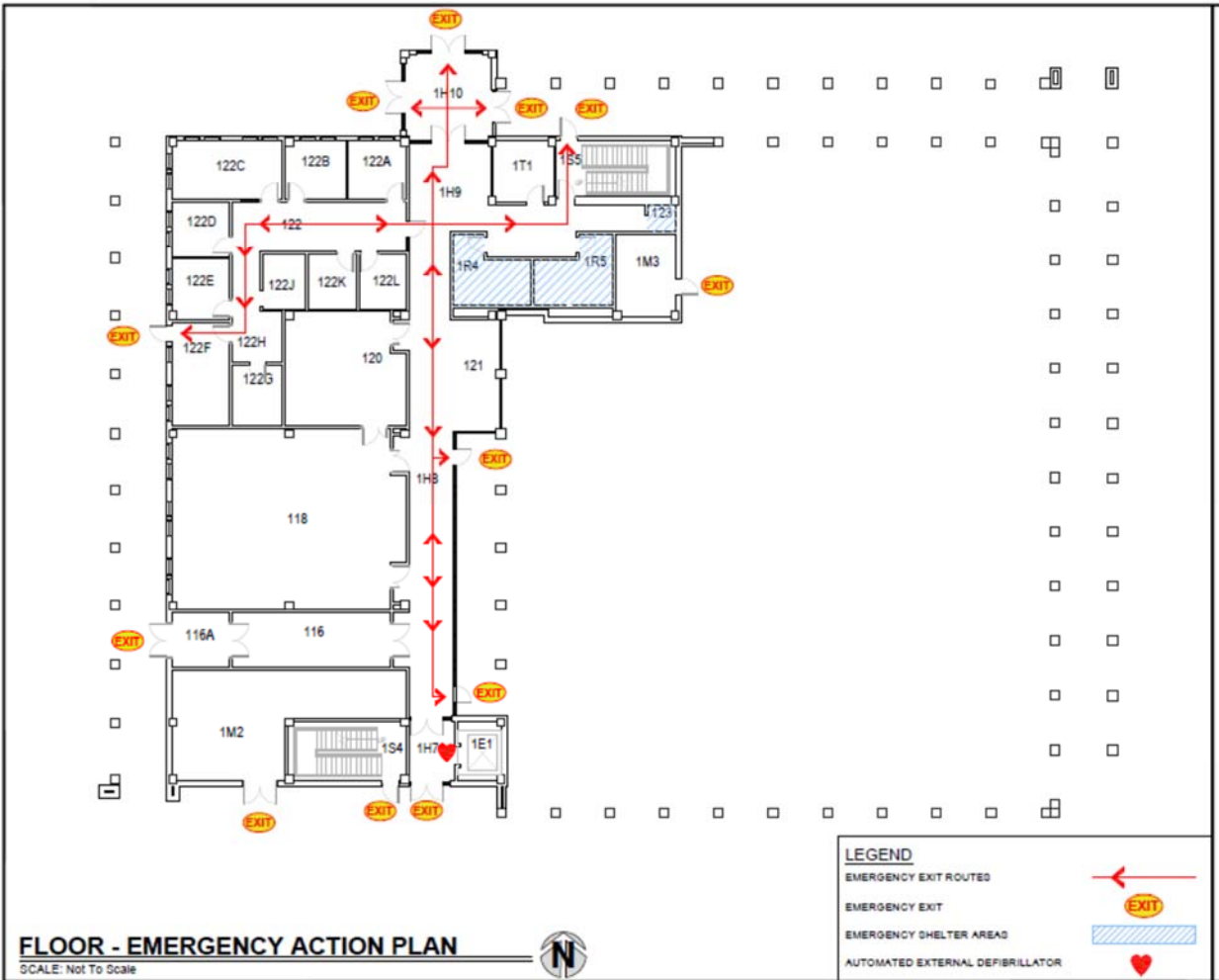
Figure 1 Bayer Plant Sciences West Building First Floor
