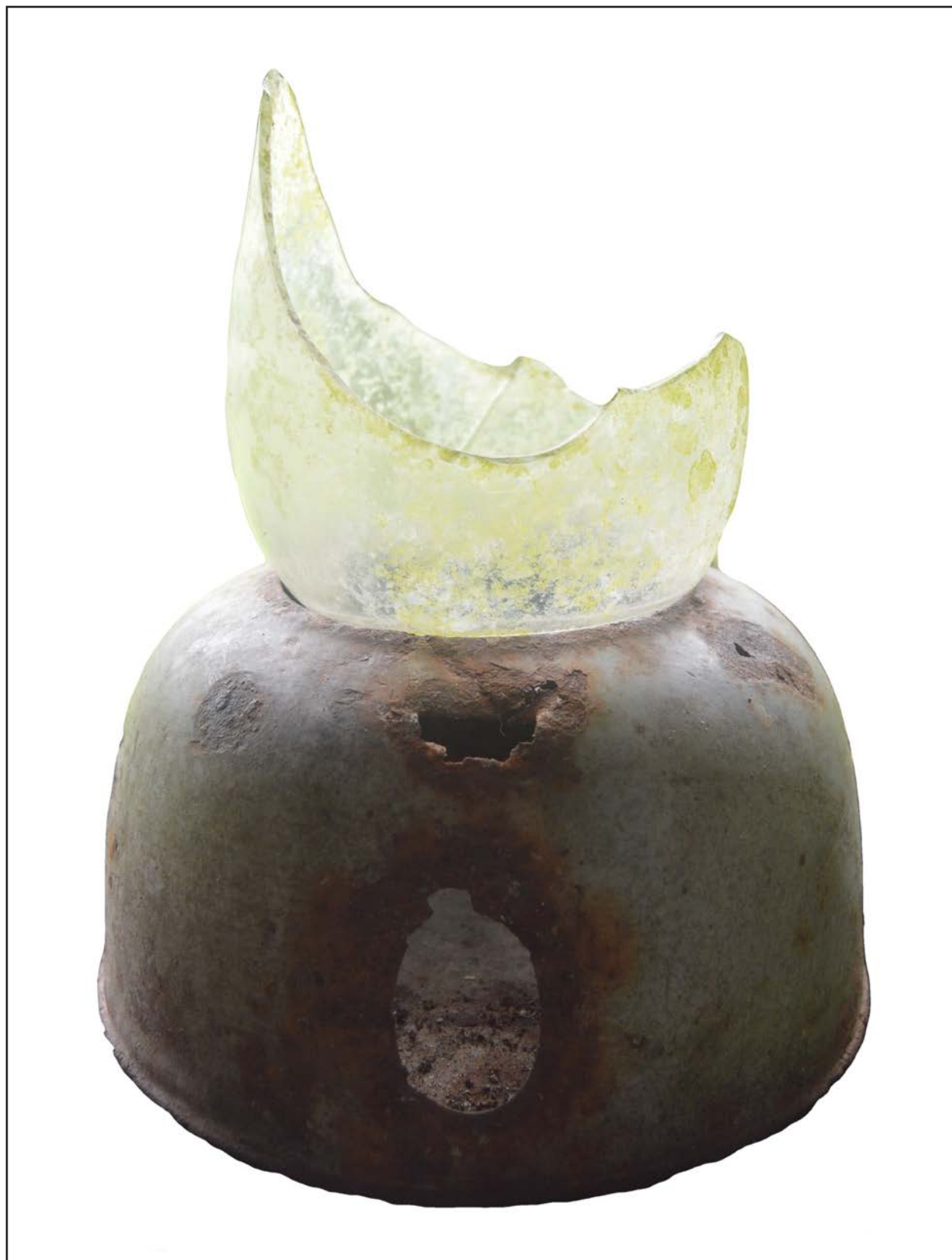
Figure 4.20. Lantern glass (Spec. # KUV1479-01) placed in metal base (Spec. # KUV1518-01). The base has a diameter of 19.3 cm.
