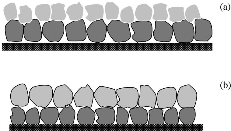
Figure 9. Aggregate Grade Combinations Used in 2-CST (a) Grade 4 on Grade 3 (b) Grade 3 on Grade 4.
