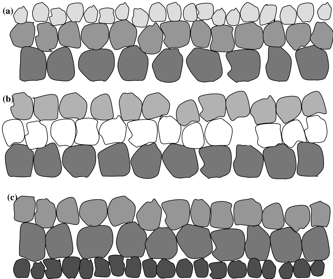
Figure 10. Aggregate Grade Combinations Used in 3-CST (a) Grade 5 on Grade 4 on Grade 3 (b) Grade 4 on Grade 4 on Grade 3 (c) Grade 4 on Grade 3 on Grade 5.
