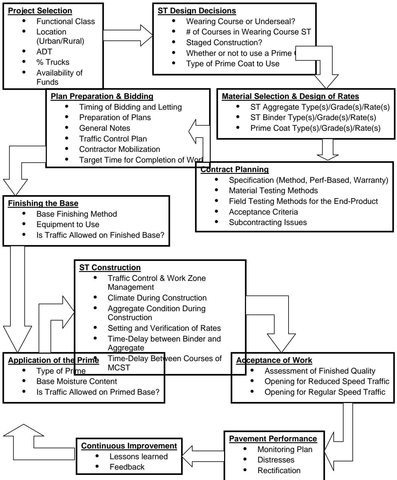
Figure 14. System component chart for design and construction of surface treatments
