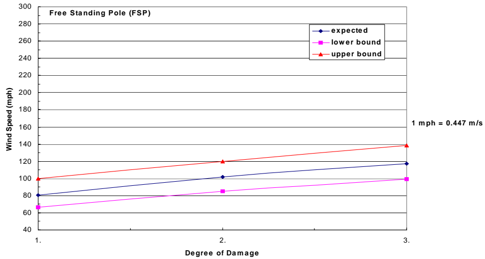
Figure 25. Wind Speed vs. Degree of Damage
