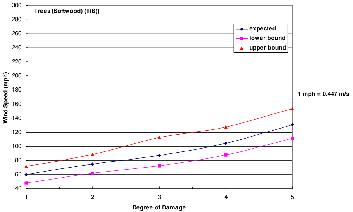
Figure 27. Wind Speed vs. Degree of Damage
