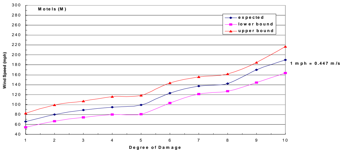
Figure 6. Wind Speed vs. Degree of Damage
