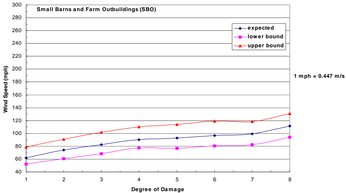
Figure 1. Wind Speed vs. Degree of Damage
