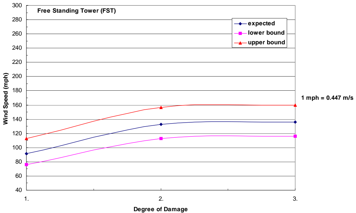
Figure 24. Wind Speed vs. Degree of Damage
