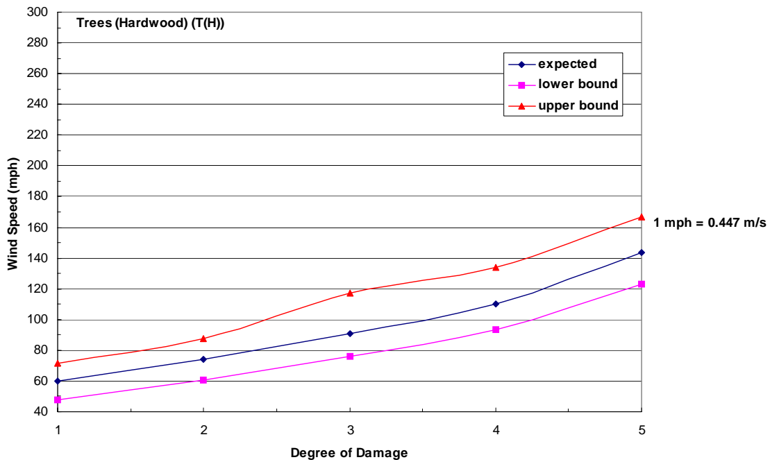
Figure 26. Wind Speed vs. Degree of Damage
