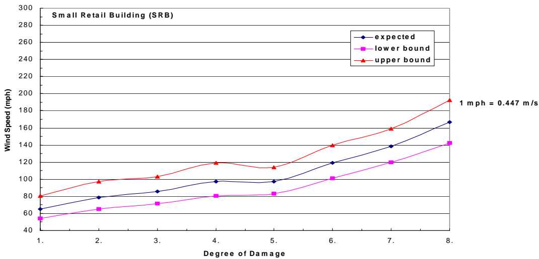
Figure 8. Wind Speed vs. Degree of Damage
