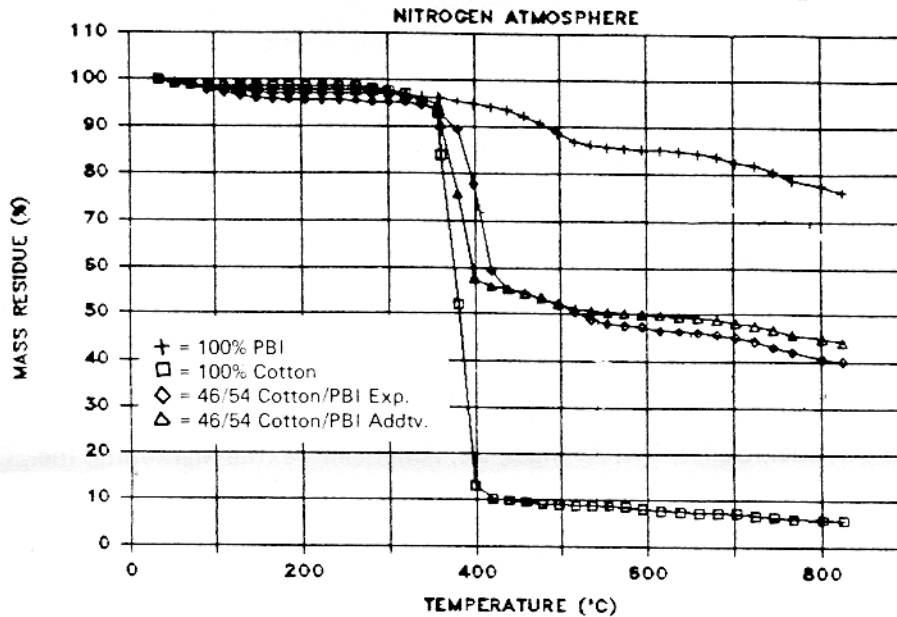
FIGURE 2: EXPERIMENTAL AND ADDITIVE TG CURVES OF 46/54 COTTON/PBI BLEND
