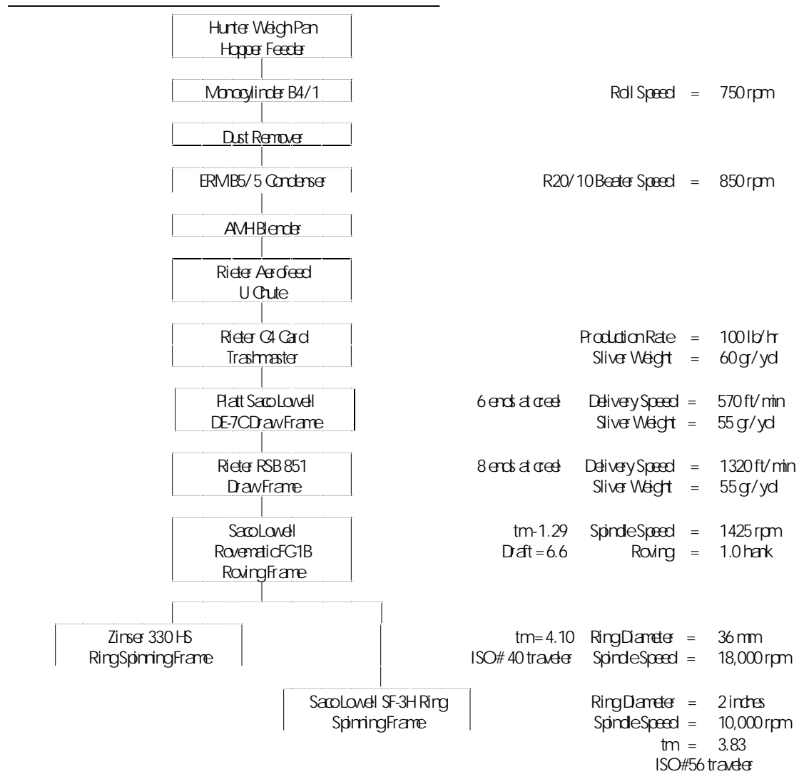
Exhibit 2: Outline of mechanical process
