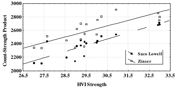
Exhibit 7. CSP vs. HVI Strength (Scatter Plots & Best-Fitting Lines)
