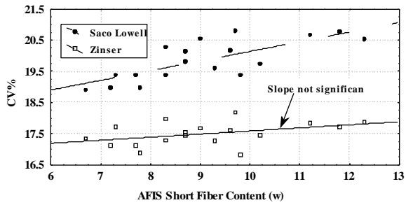
Exhibit 9. Yarn Non-Uniformity vs. AFIS Short Fiber Content (Scatter Plot & Best-Fitting Lines)
