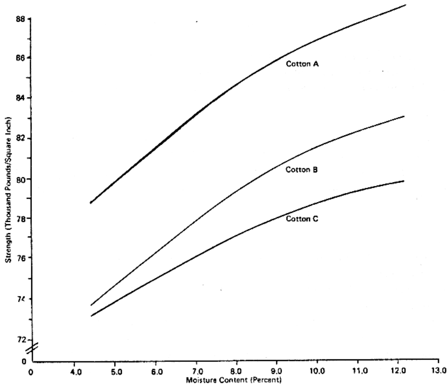
Fiber Strength at Specified Percentages of Moisture Content
