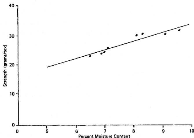
Moisture Content of the Cotton Fiber and Strength in grams/tex
