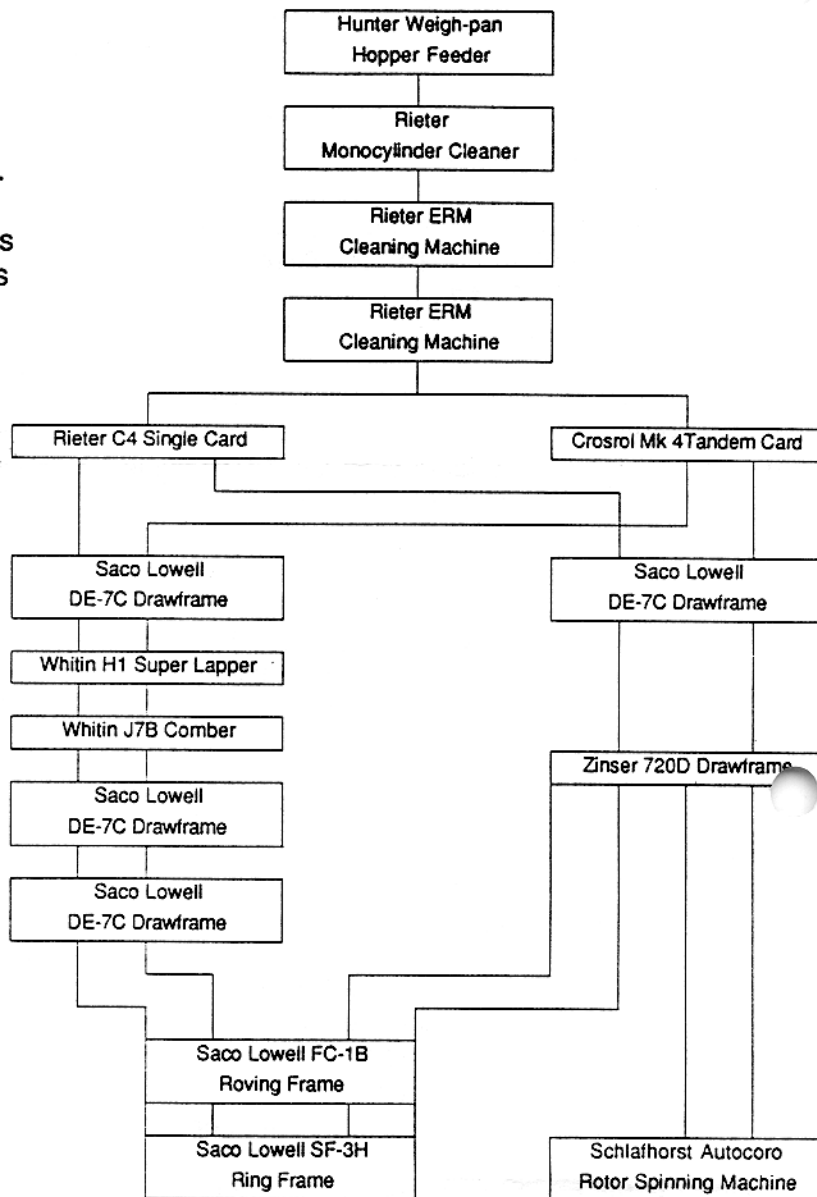
FIGURE 1 MATERIAL PROCESSING ROUTES
