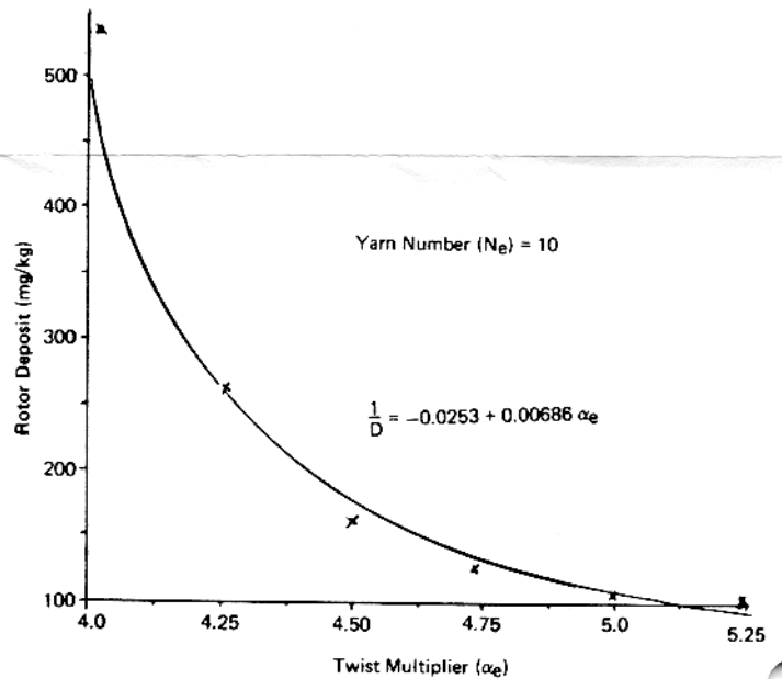
FIGURE 4: INFLUENCE OF YARN TWIST ON ROTOR DEPOSIT
