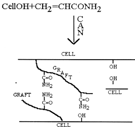
Exhibit 1: Graft polymerization of acrylamide on cotton fiber
