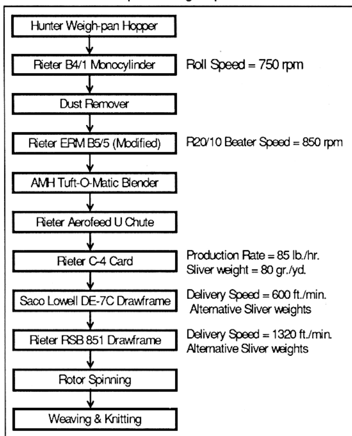
Exhibit 2: Outline of processing steps
