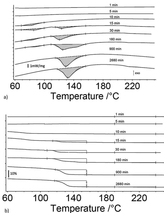
Fig. 1 (a) DSC measurements of heat flow for 17 μm I_2O_5 at different exposure time intervals to 80% RH as indicated on the curves; and, (b) TG measurements of mass change for 17 μm I_2O_5 at different exposure time intervals to 80% RH as indicated on the curves. Onset and end temperature for measurements of mass loss are determined by endotherm onset and end temperatures.
