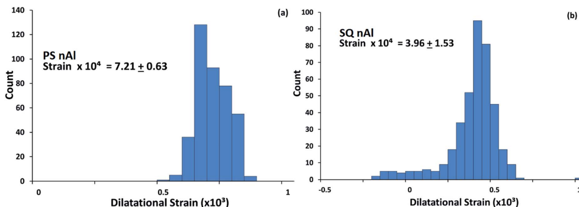
Fig. 2 Distribution of dilatational strain for (a) PS nAl and (b) SQ nAl particles, with average dilatational strain and standard deviation indicated in each figure.
