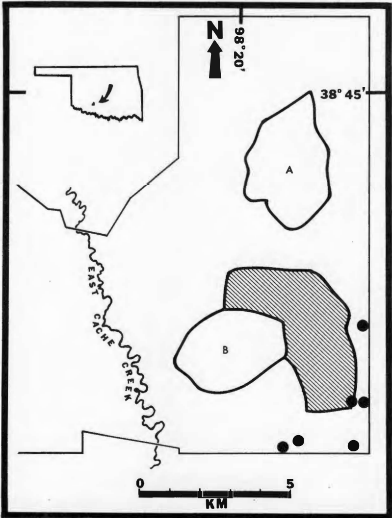
FIG. 1.—Study site, east range of Fort Sill, Oklahoma. Hatched area represents the Tall Grass Prairie Preserve. A and B indicate the north and south impact areas, respectively. Trapping locations are marked with black circles.
