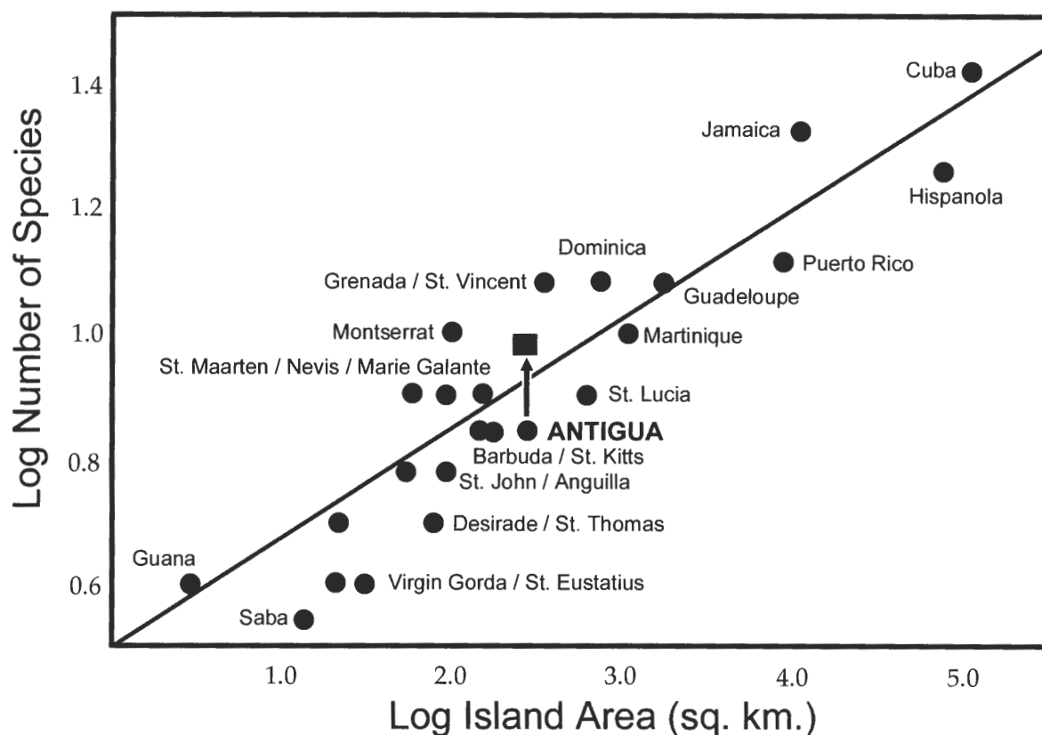
Figure 2. Species/area curve for the chiropteran fauna in the Antilles. Data are from Genoways et al. (2001) with minor modification. Linear regression of log-transformed data: y = 0.17x + .49 ( R\text{-squared} = 0.81 ). For argument (see text), Antigua has been represented twice with the extant compliment of seven species of bats (closed circle) and with its compliment increased by three additional species (Arrow: Square).
