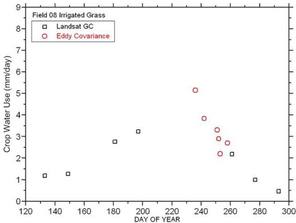
Figure 19. Estimated (from Landsat ground cover) and observed (EC) daily CWU for irrigated grass Field 8.
