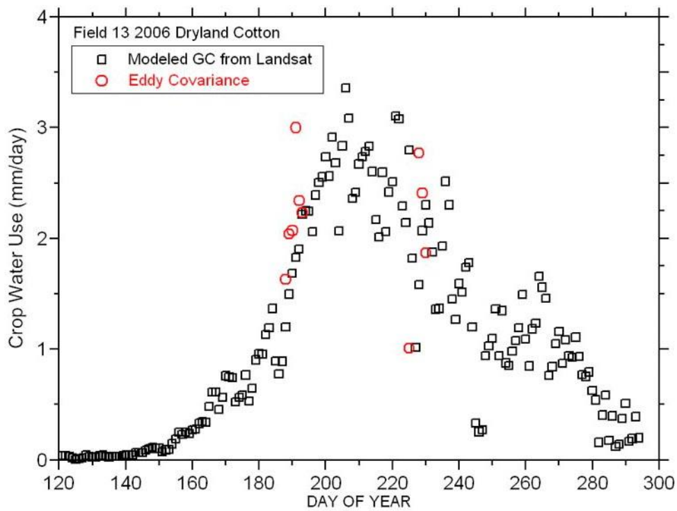
Figure 17. Modeled and observed daily CWU for the dryland cotton Field 13.
