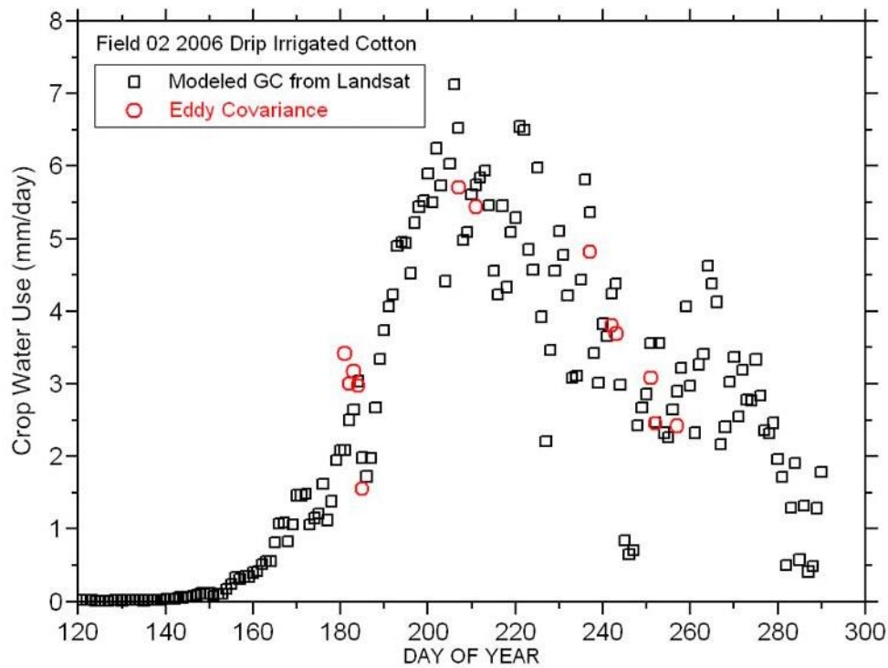
Figure 16. Modeled and observed daily CWU for the drip-irrigated cotton Field 2.
