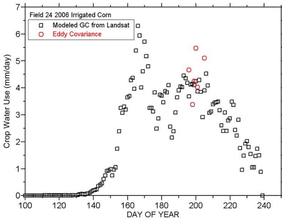
Figure 18. Modeled and observed daily CWU for the irrigated corn Field 24.
