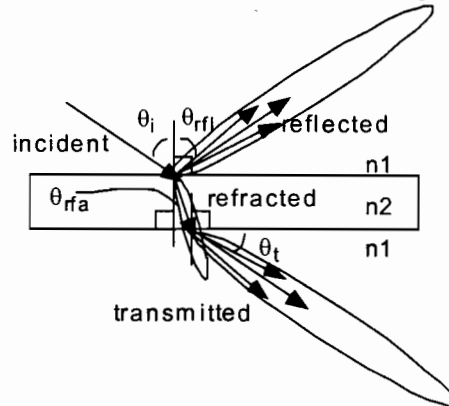
Figure 2.5. Reflection and Transmission Distributions
