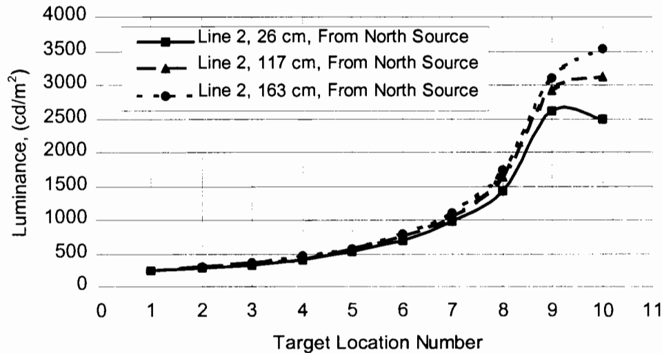
Figure 6.27 Luminance distribution, from north source, at 26 cm, 117 cm and 163 cm height above the roadway surface on line 2.
