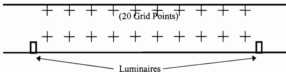
Figure 2.10. Network of Grid Points Between Luminaires Used to Calculate STV
