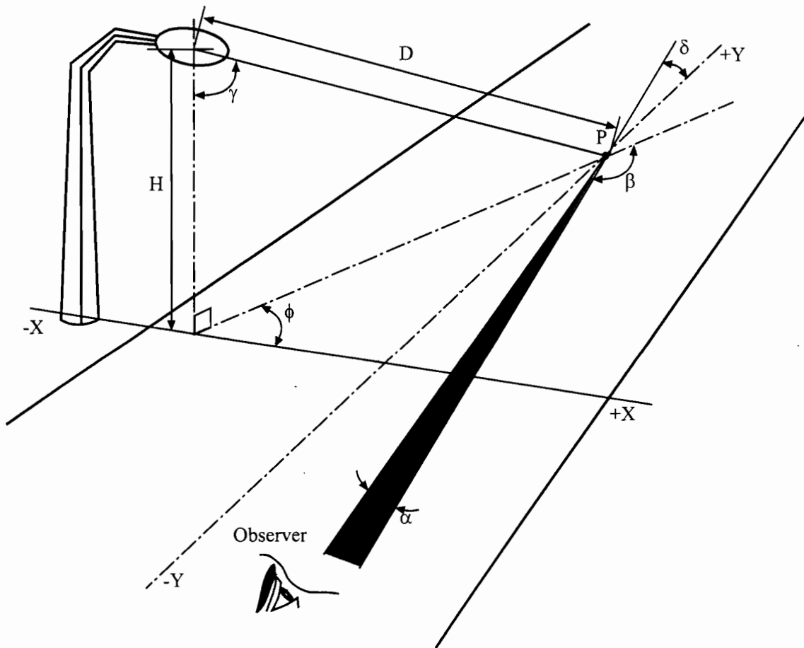
Figure 7.8 Single luminaire.
