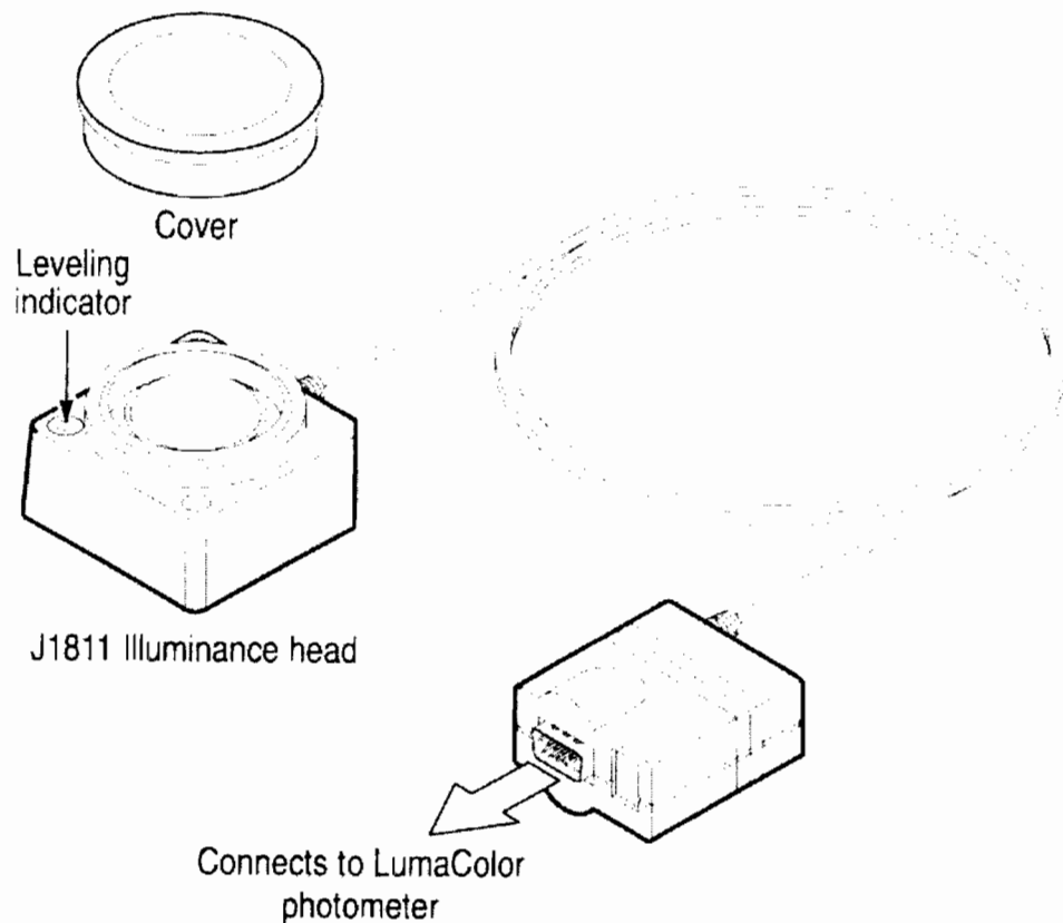
Figure 5.4 Illuminance probe.
