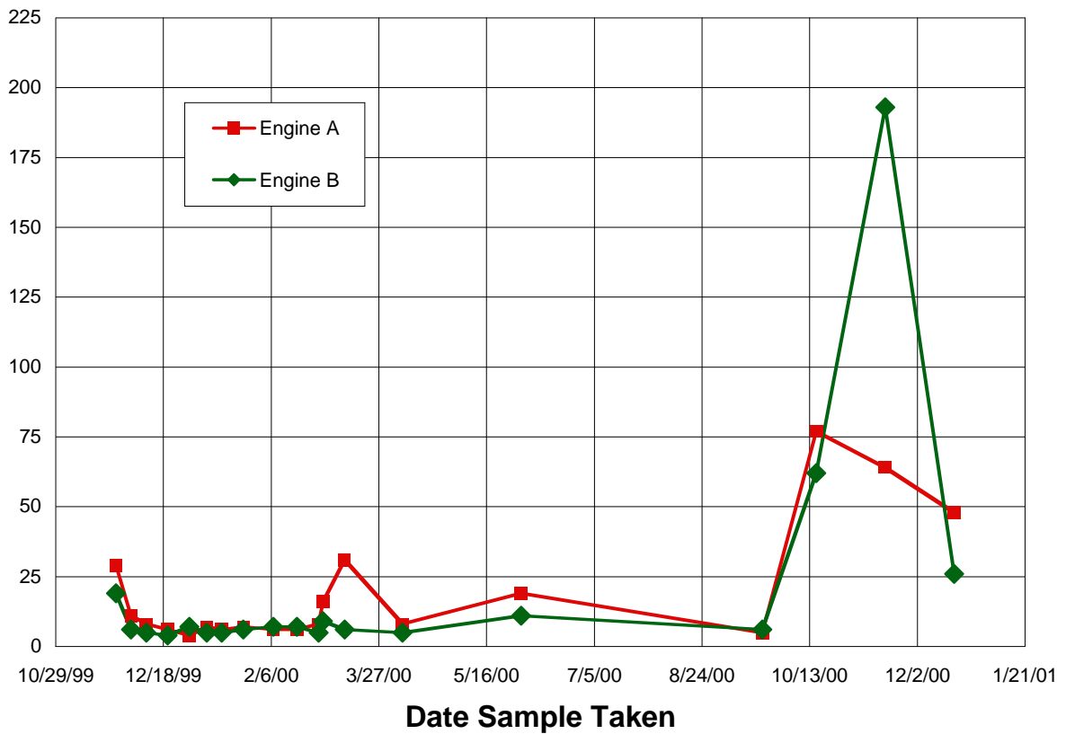
Figure A.14 Sodium Concentration for Engine Oil Samples
