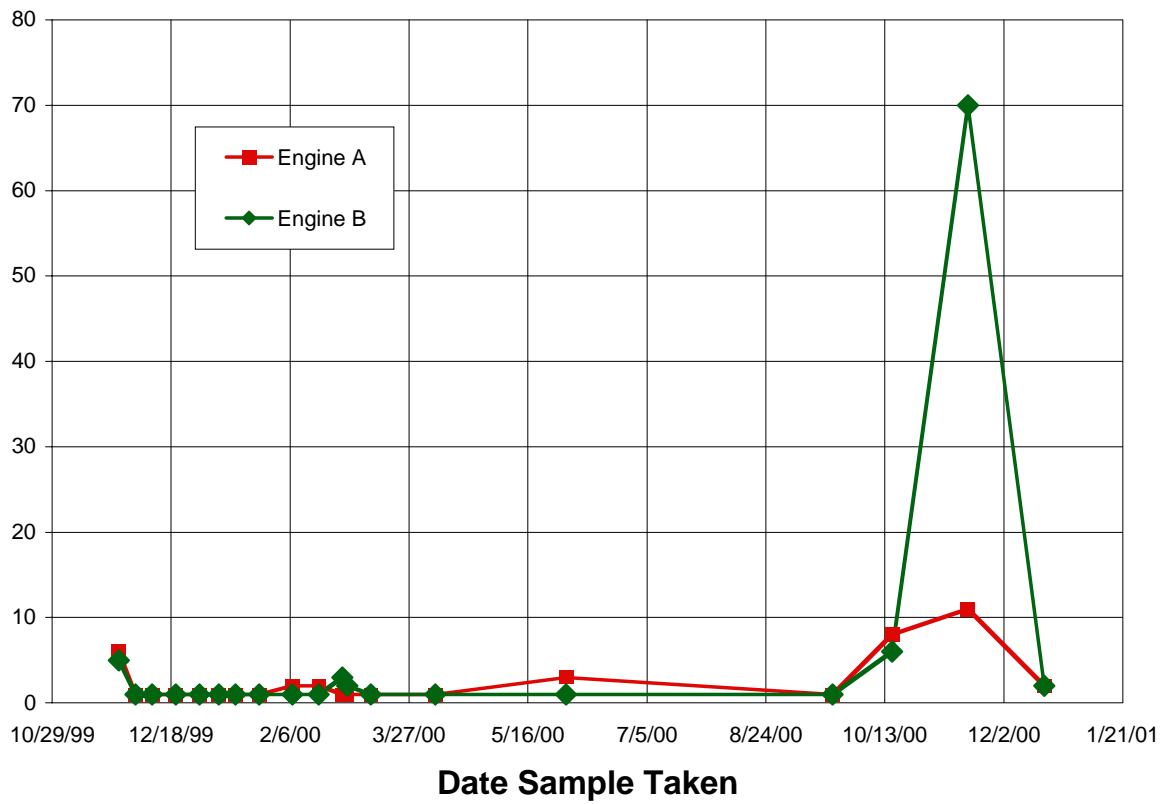
Figure A.8 Lead Concentration for Engine Oil Samples
