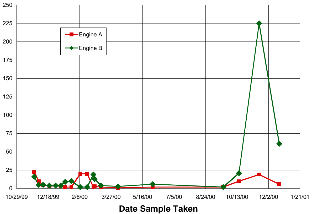
Figure A.9 Aluminum Concentration for Engine Oil Samples
