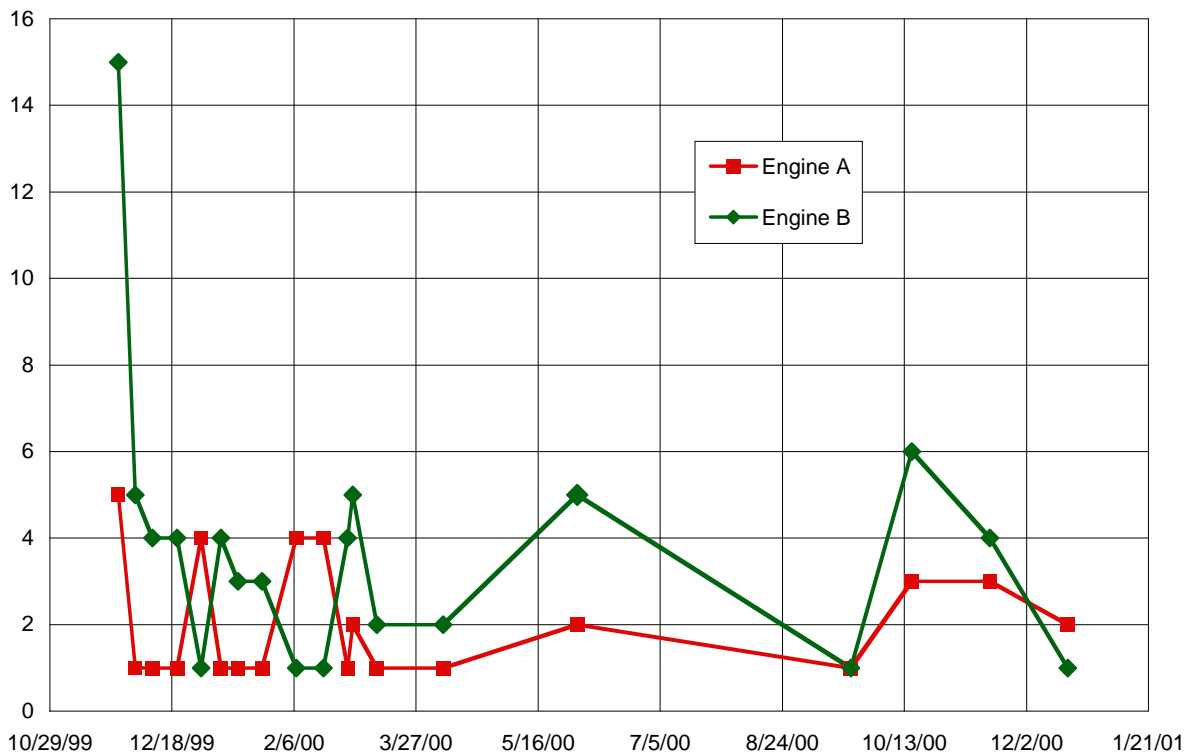
Date Sample Taken Figure A.7 Chromium Concentration for Engine Oil Samples
