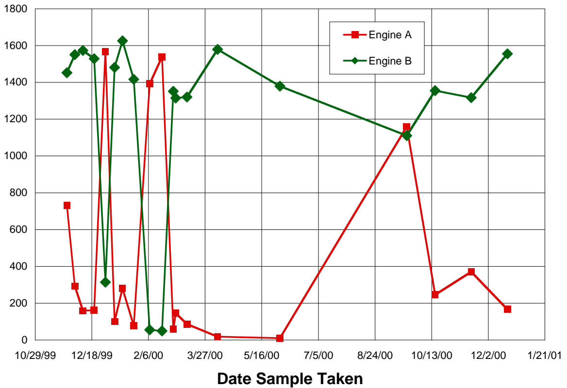
Figure A.15 Phosphorus Concentration for Engine Oil Samples
