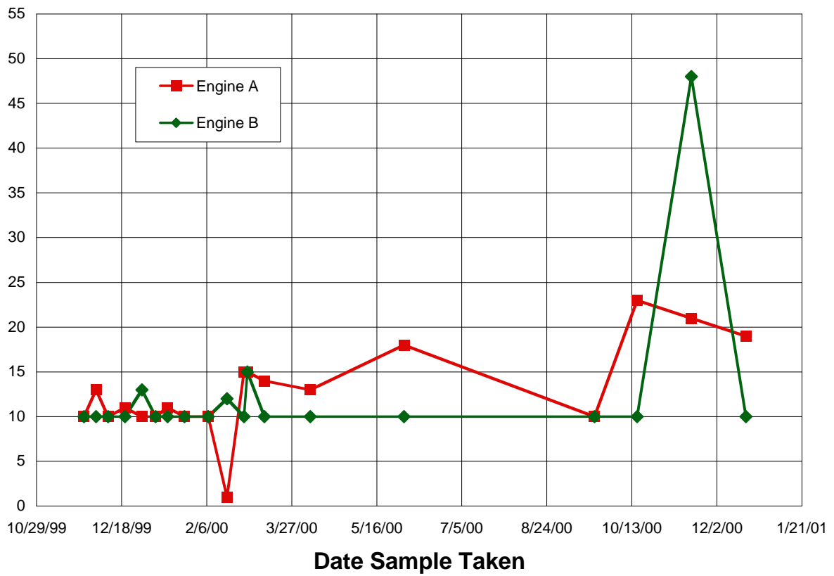
Figure A.12 Potassium Concentration for Engine Oil Samples
