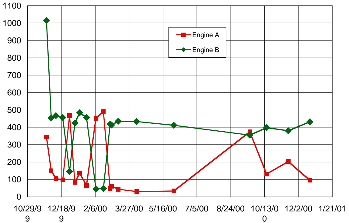
Date Sample Taken Figure A.6 Magnesium Concentration for Engine Oil Samples
