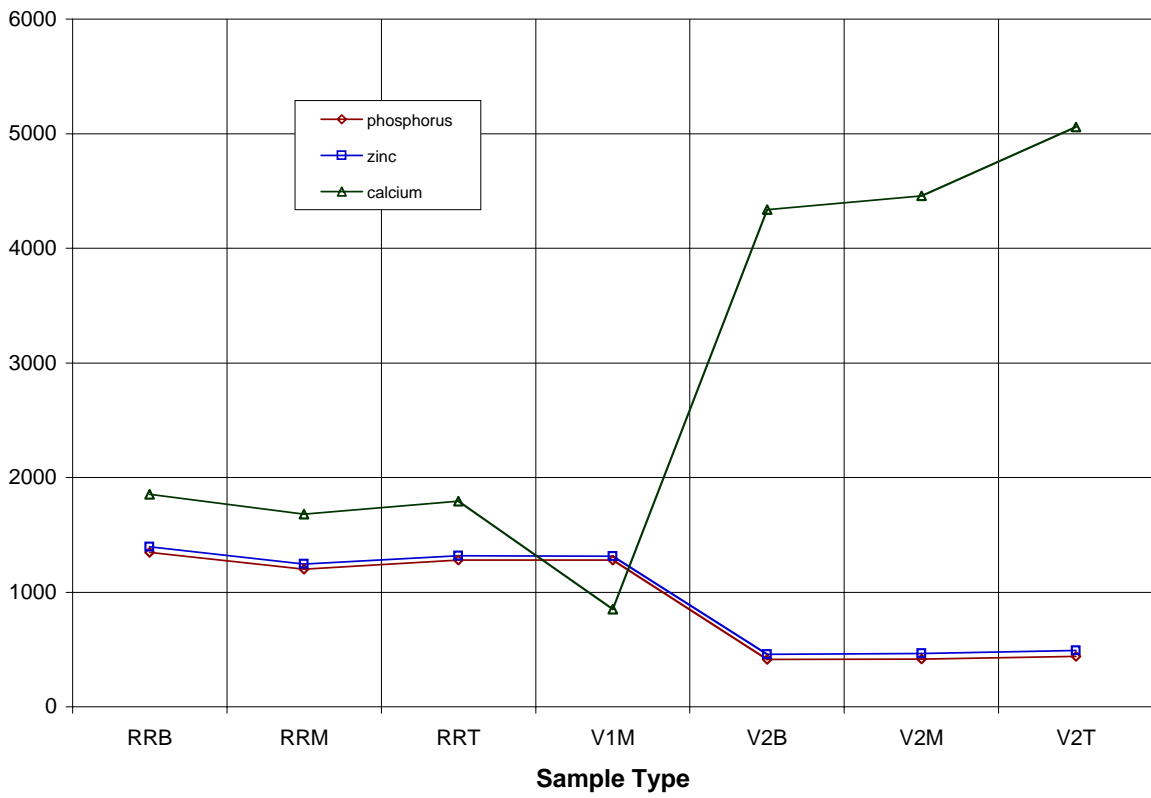
Figure A.2 Species Concentrations for Reference Oils
