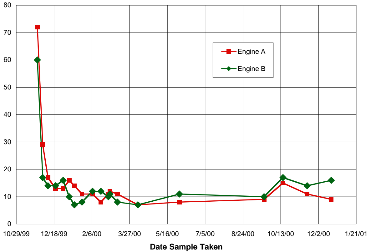
Figure A.10 Silicon Concentration for Engine Oil Samples
