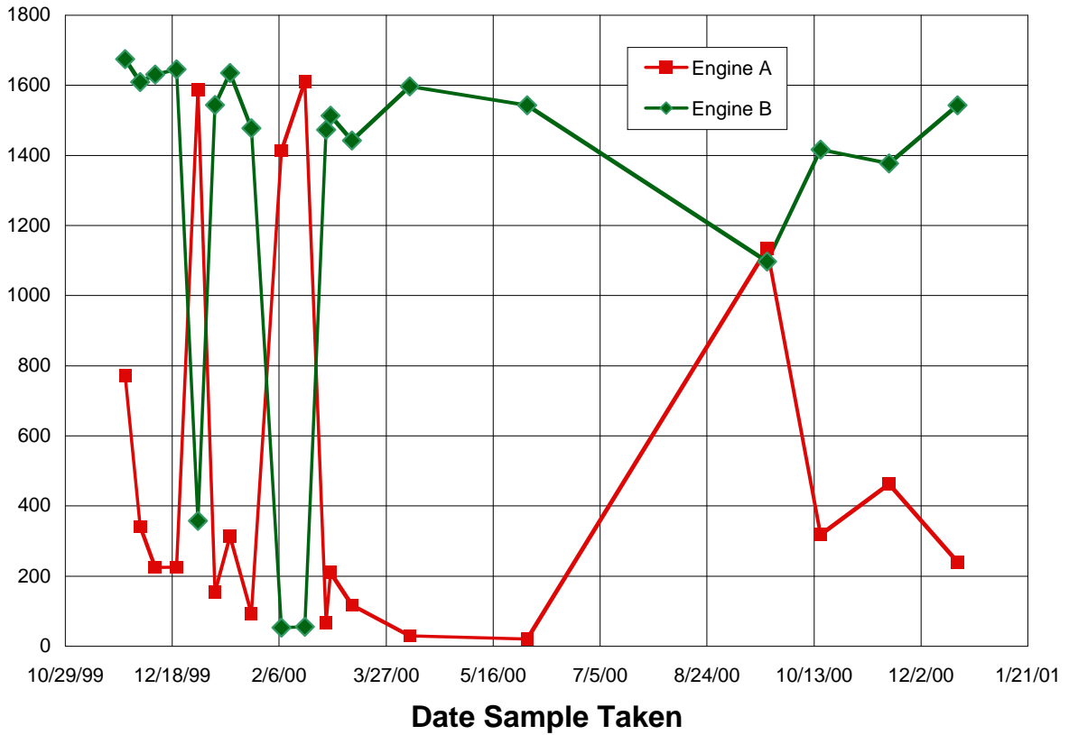
Figure A.16 Zinc Concentration for Engine Oil Samples
