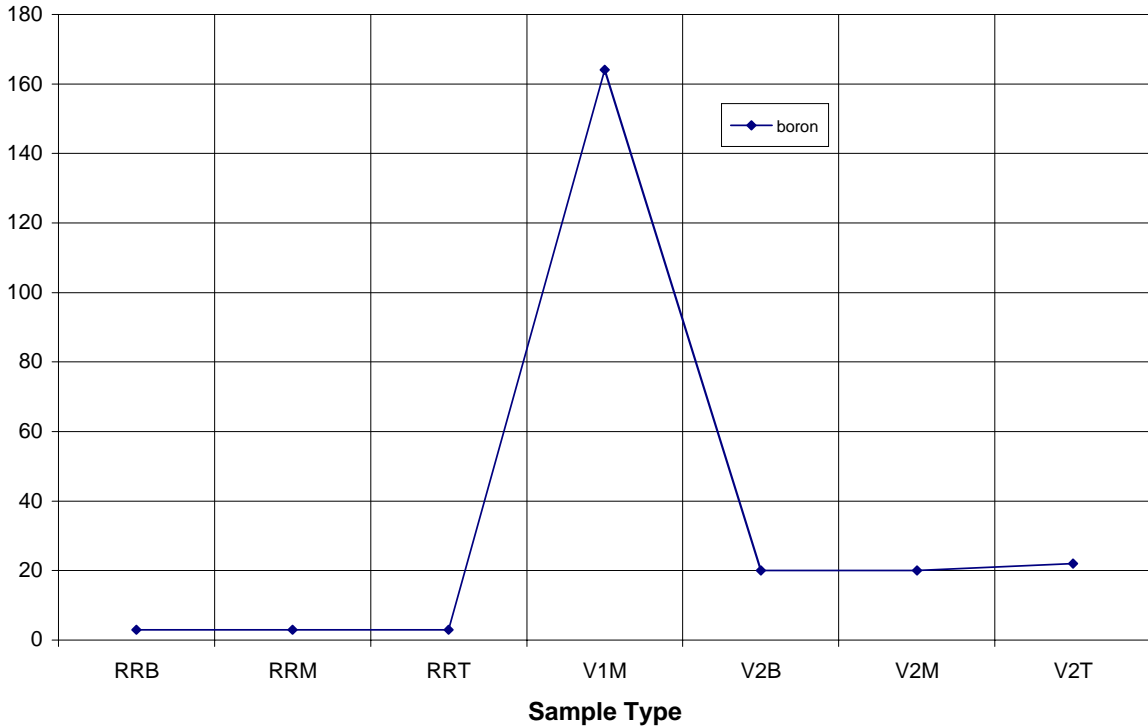
Figure A.1 Species Concentrations for Reference Oils
