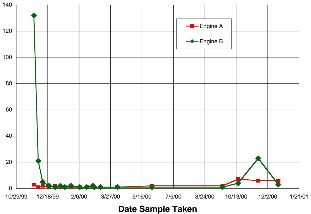
Figure A.11 Boron Concentration for Engine Oil Samples
