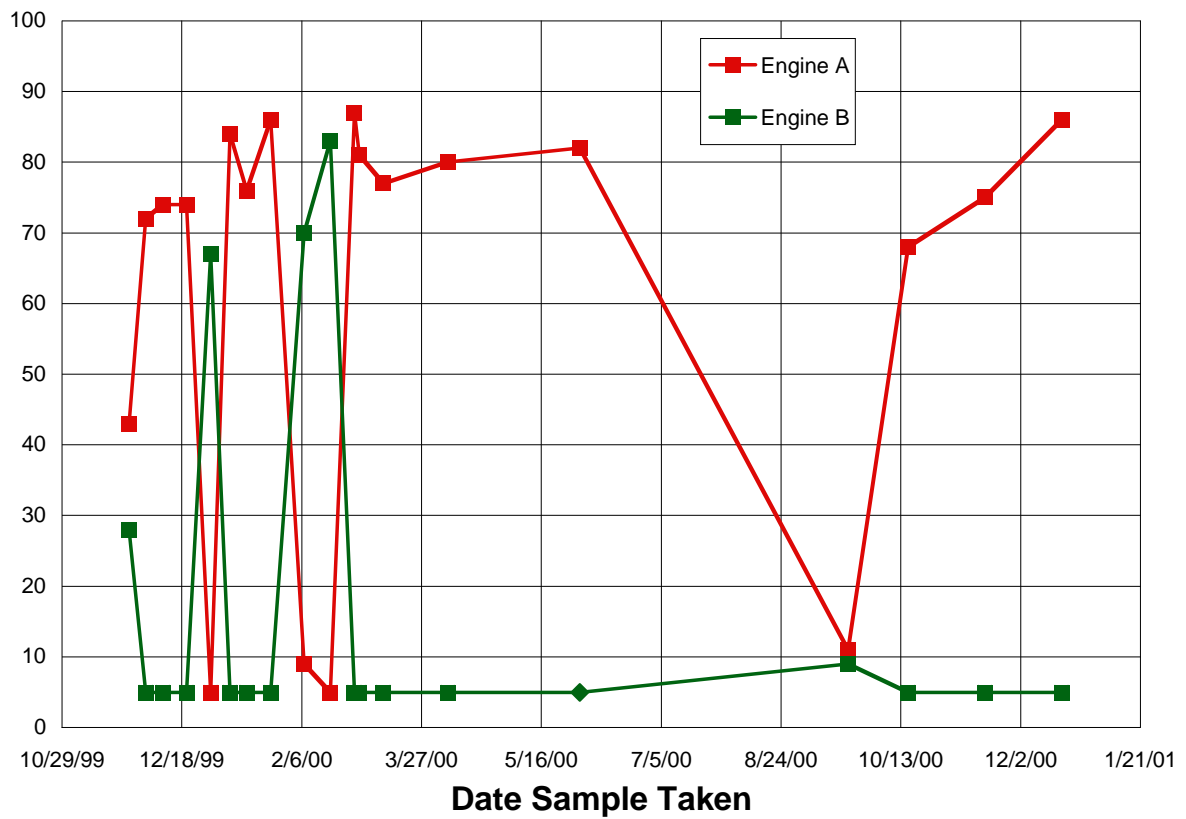
Figure A.13 Molybdenum Concentration for Engine Oil Samples
