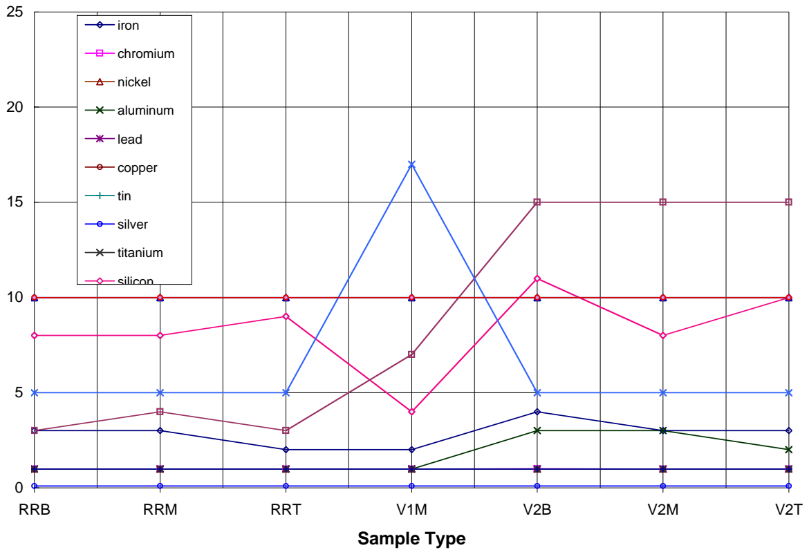
Figure A.3 Species Concentrations for Reference Oils
