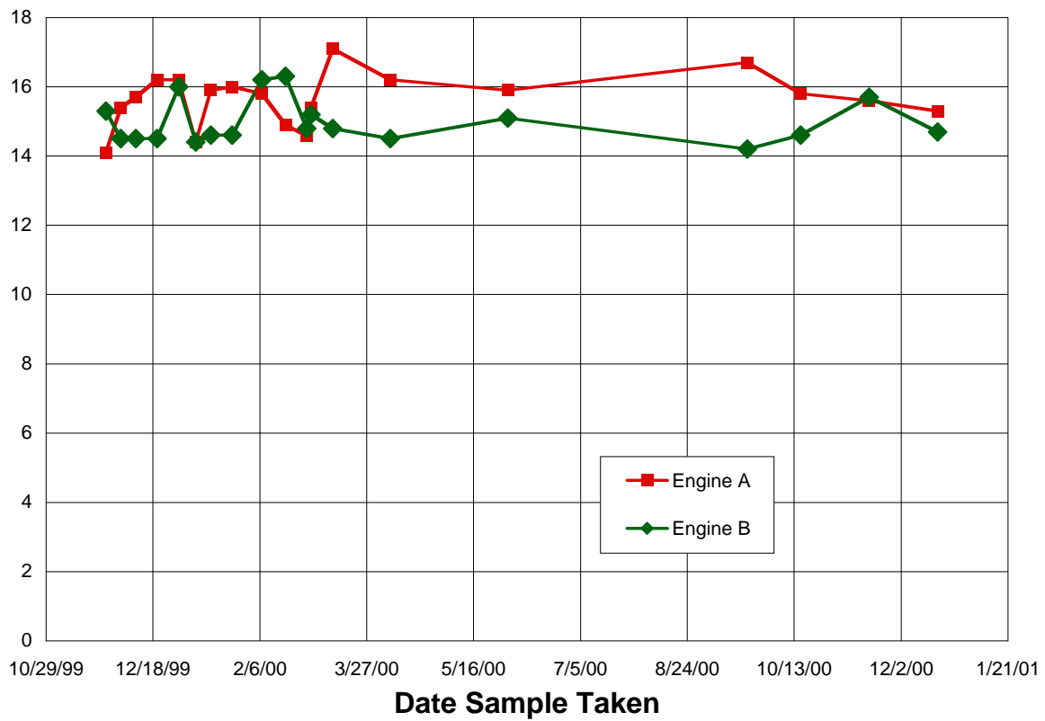
Figure A.18 Viscosity for Engine Oil Samples
