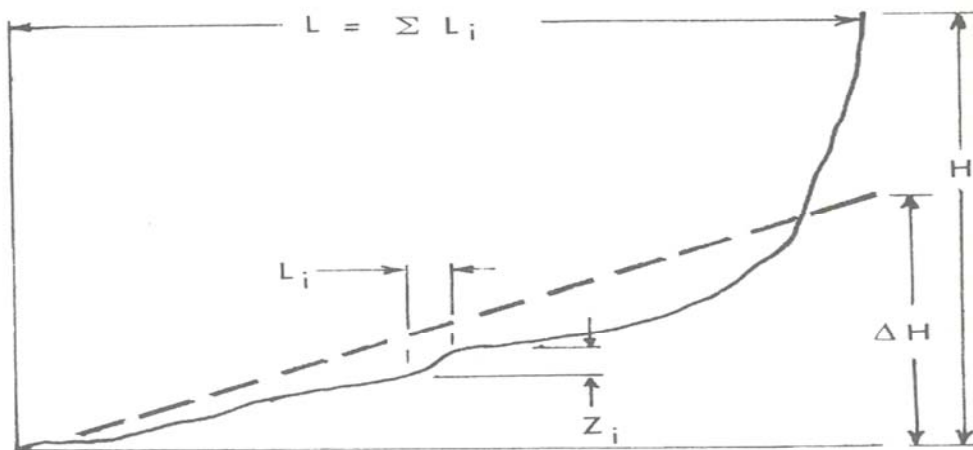
Figure 4.2. Definition of average main channel slope (from Schulz and Lopez, 1974).
