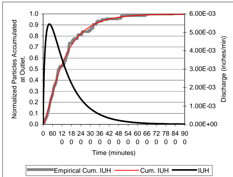
Figure A.17 Empirical and fitted IUH for Slaughter Creek.
