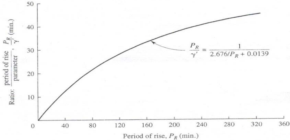
Figure 3.5. Relation for storage factor, P_R / \gamma' , and period of rise P_R (after Gray, 1961).
