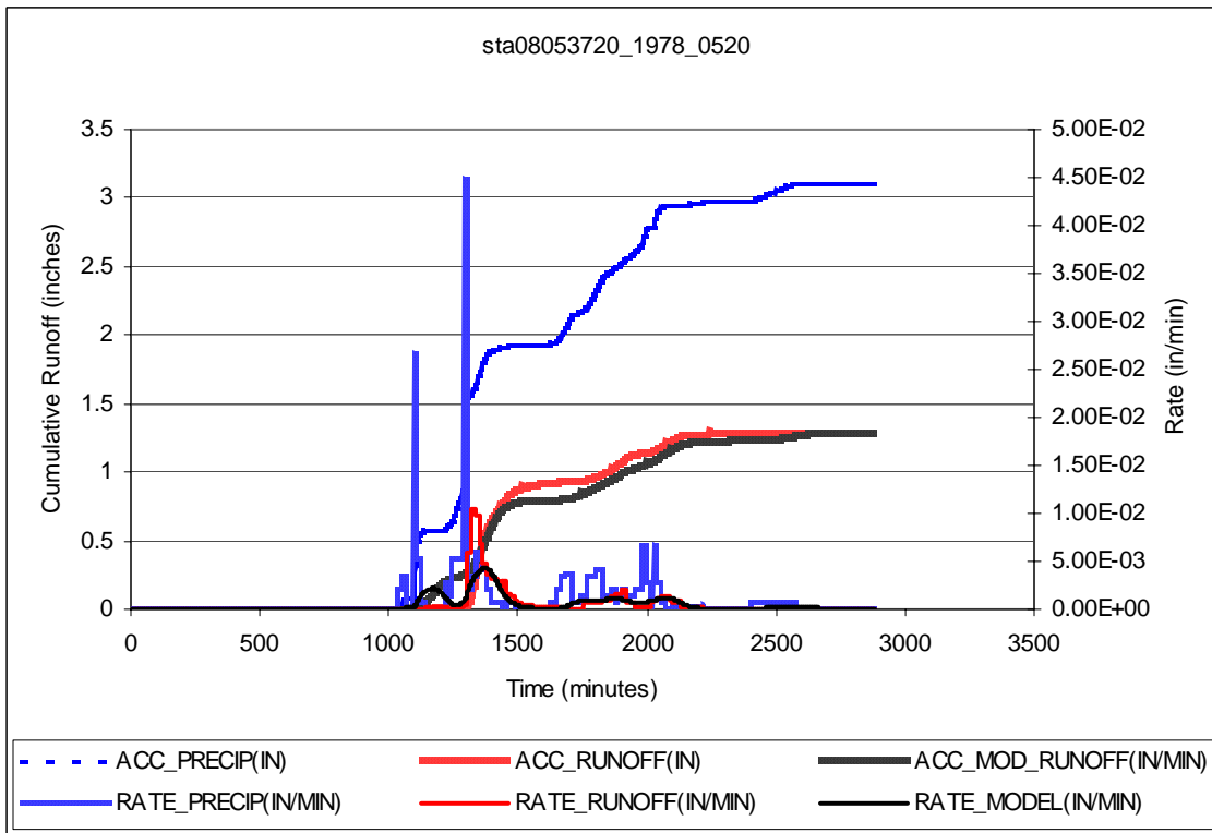
Figure A.14 Ash Creek response under rainfall on 05-20-1978.
